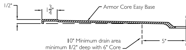
Threshold Detail
